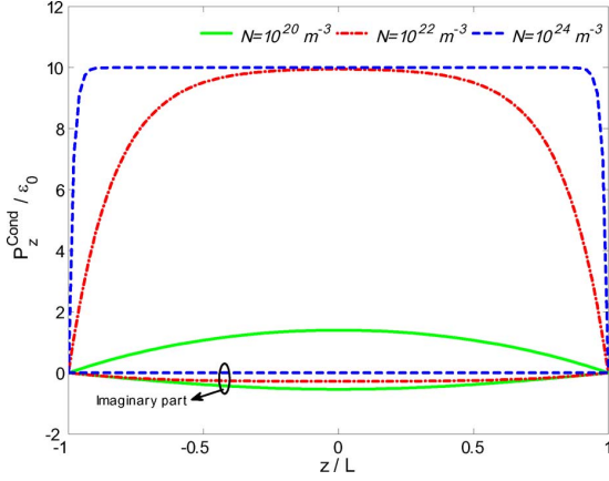
Fig. 5. Conductive part of the polarization for a semiconductor with E^{\text{inc}} = 10 V/m, f = 10 GHz, L = 250 nm, T = 300 K, \tau = 2.16 \times 10^{-13} s, \varepsilon_h = 11.9 , and m_{eff} = 0.26m_e , for charge (doping) number density N = 10^{20} , 10^{22} , and 10^{24} \text{m}^{-3} . Higher doping leads to better screening.
