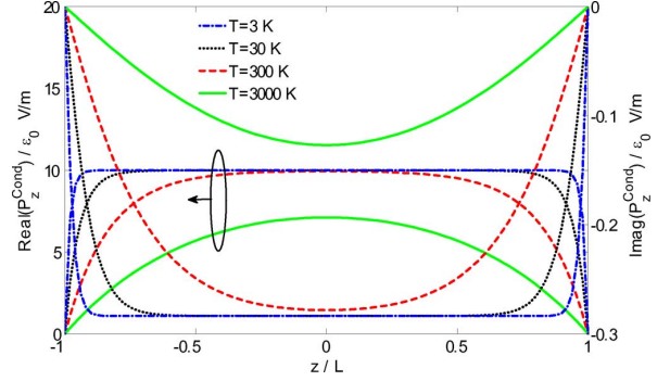
Fig. 6. Conductive part of the polarization for a semiconductor with E^{\text{inc}} = 10 V/m, f = 10 GHz, L = 250 nm, \tau = 2.16 \times 10^{-13} s, \varepsilon_h = 11.9 , and m_{eff} = 0.26m_e , for charge (doping) number density N = 10^{22} \text{m}^{-3} at several different temperatures. Higher temperature leads to more diffusion.
